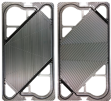
Cooling water side Vapor side YX-83 plate
