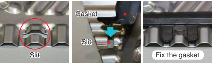
Installation of Slit-in Gaskets
