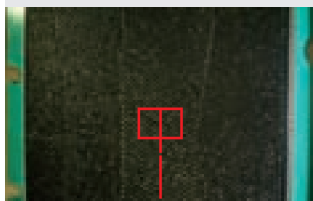
↑ Heat exchanger Seawater inlet port hole Wood chips, seaweeds and shellfish are blocking the flow channel, and causing poor flow in the unit.
