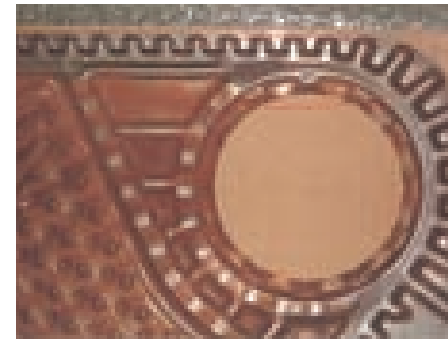
← Port hole (from the back side of the plate) can be seen to be severely deformed.
