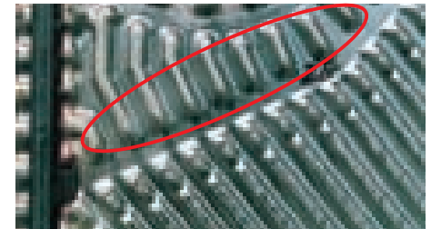
↑ Erosion corrosion at the plate contact points and near contact points
