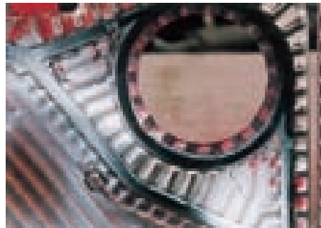
↑ Penetration cracking in red areas (the developing fluid by DPT)
