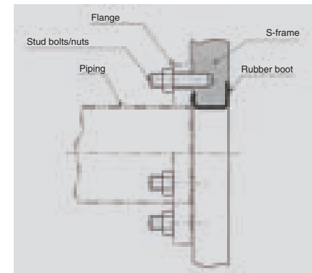
↑ For a rubber boot type, a piping gasket is not necessary.
