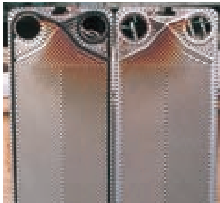
↑ Steam side
